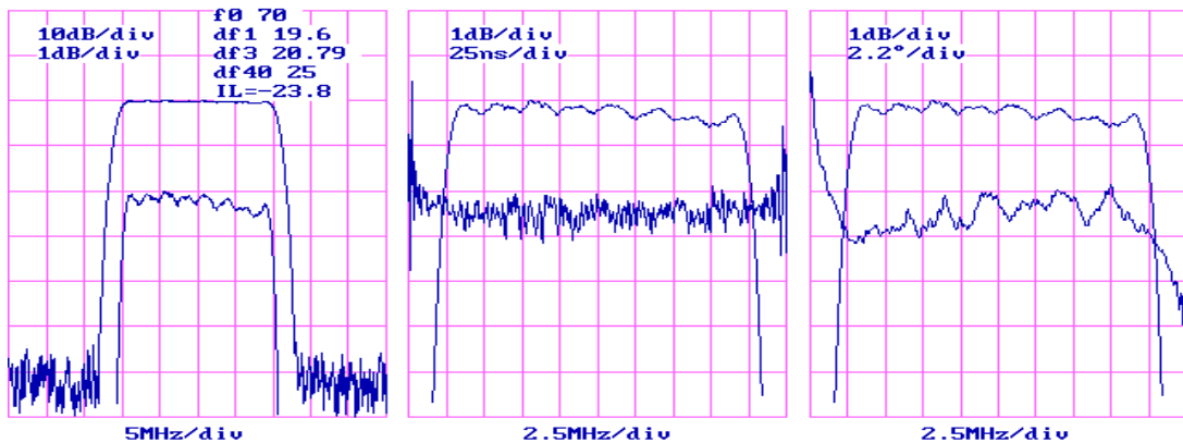
LBN7011 SAW Filter Typical Performance
