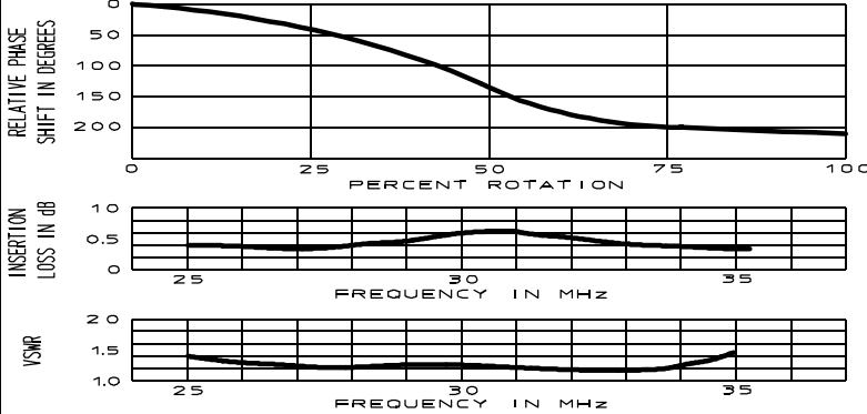
Typical Performance
