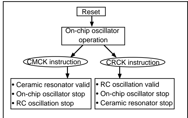
Fig. 43 Switch to ceramic resonance/RC oscillation
