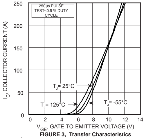
FIGURE 3, Transfer Characteristics
