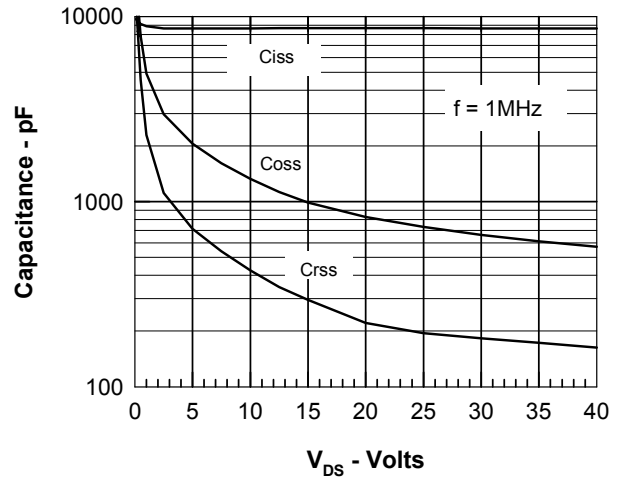
Figure 8. Capacitance Curves
