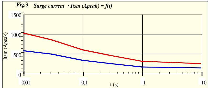
fig 3 : Courants de surcharges / Overload currents
