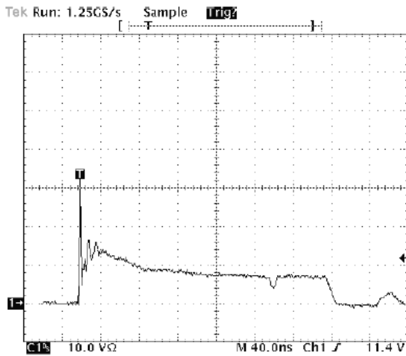
Figure 4. Positive 8kV contact per IEC 61000-4-2-LESD7D5.0T5G
