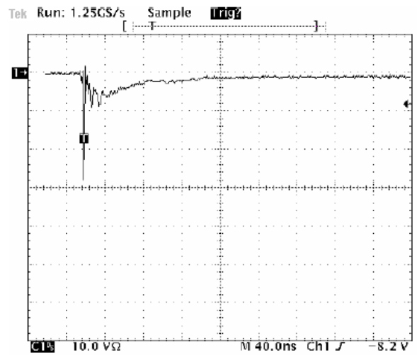
Figure 5. Negative 8kV contact per IEC 61000-4-2-LESD7D5.0T5G
