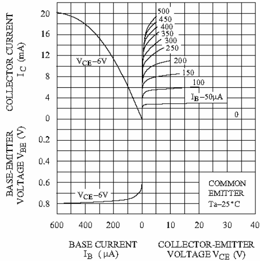
STATIC CHARACTERISTICS
