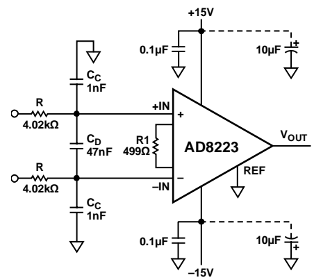
Figure 32. RFI Suppression
