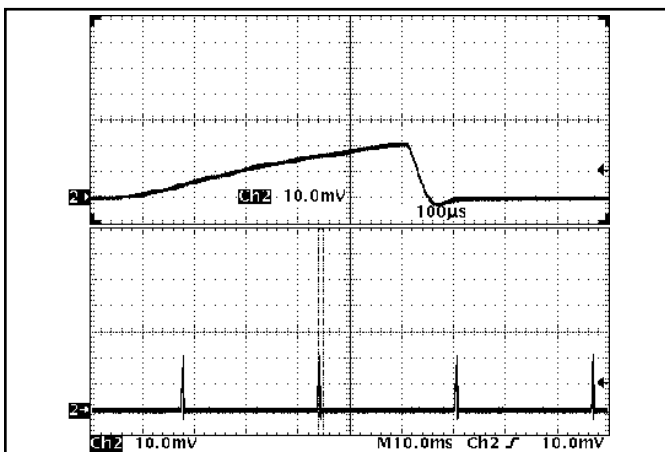
Figure 29: Load current (10A/div) as a function of time when a 3.3Vin, 0.9Vo unit attempts to turn on into a 10 m \Omega short circuit. Top trace (100 \mu s/div) is an expansion of the on-time portion of the bottom trace.
