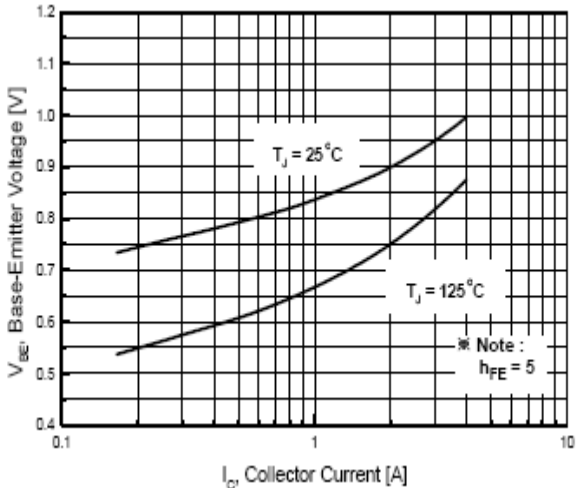
Fig. 3 Base-Emitter Saturation Voltage
