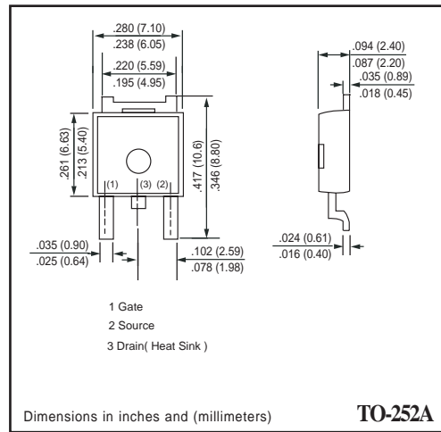
TO-252A
