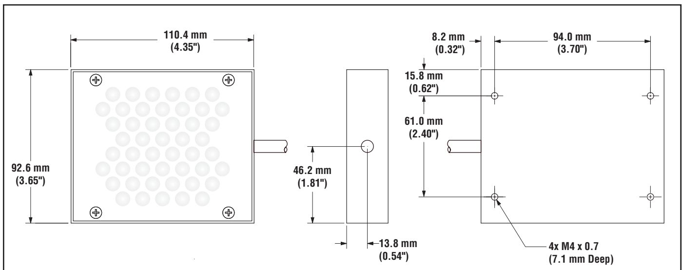
Figure 1. Model LEDRA80X80 area light dimensions
