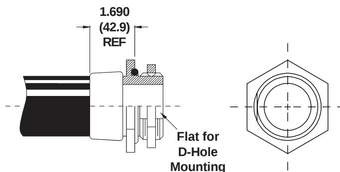
Designator T Transition Fitting
