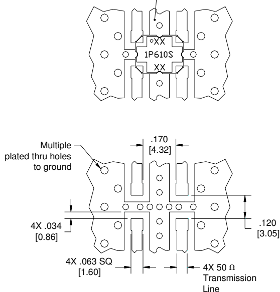
Dimensions are in Inches [Millimeters] 1P610S Rev A Mounting Footprint
