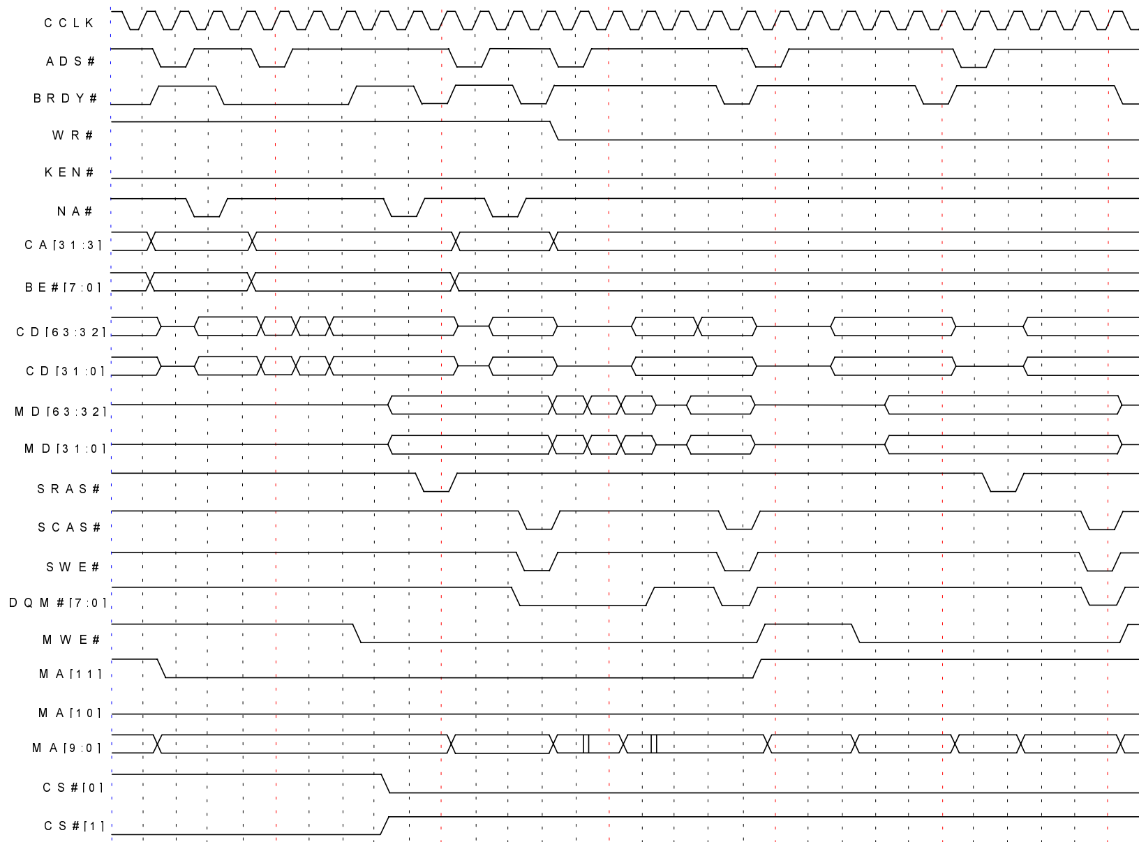
Figure 9. SDRAM WRITE CYCLE (BANK INTERLEAVE)
