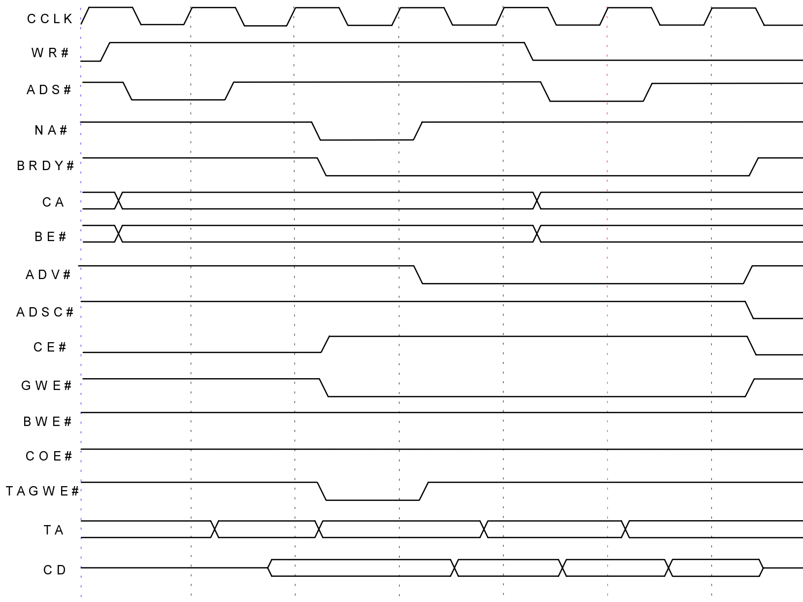
Figure 11. CPU WRITE HIT SYNCHRONOUS SRAM 3111
