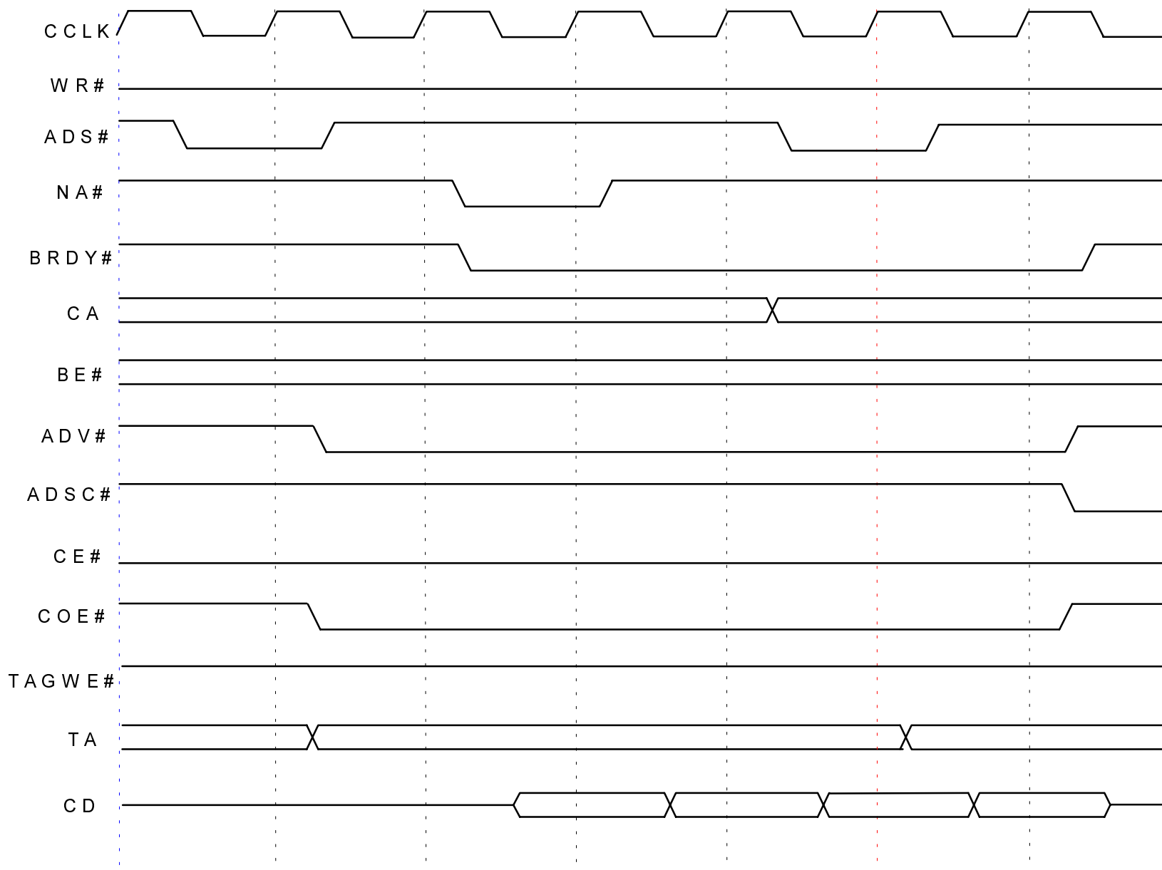
Figure 10. CPU READ HIT SYNCHRONOUS SRAM 3111
