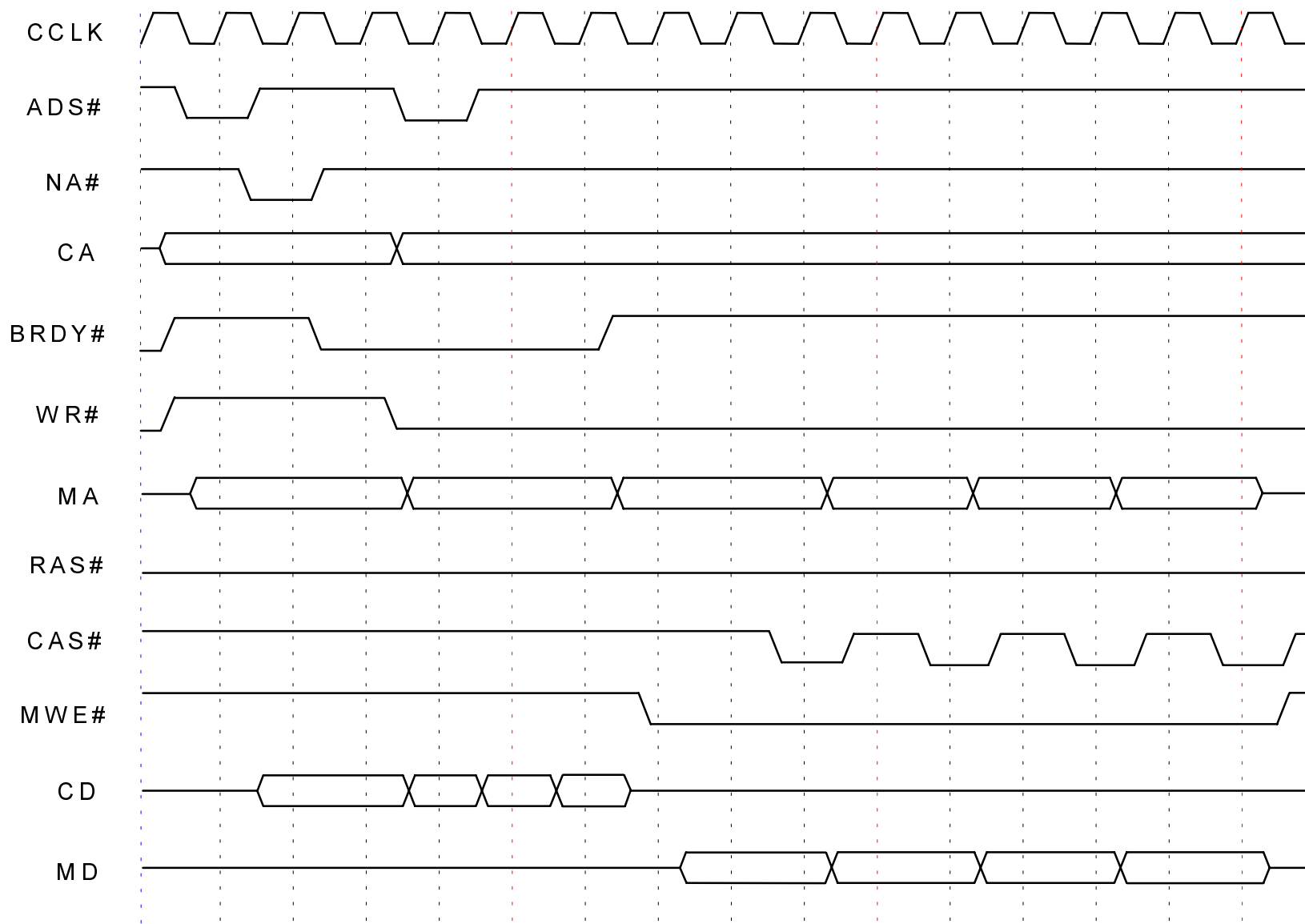
Figure 7. POST WRITE 3111, DRAM EDO 2222
