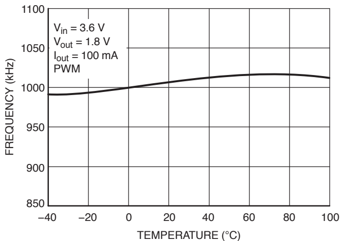
Figure 14. Oscillator Frequency vs. Temperature
