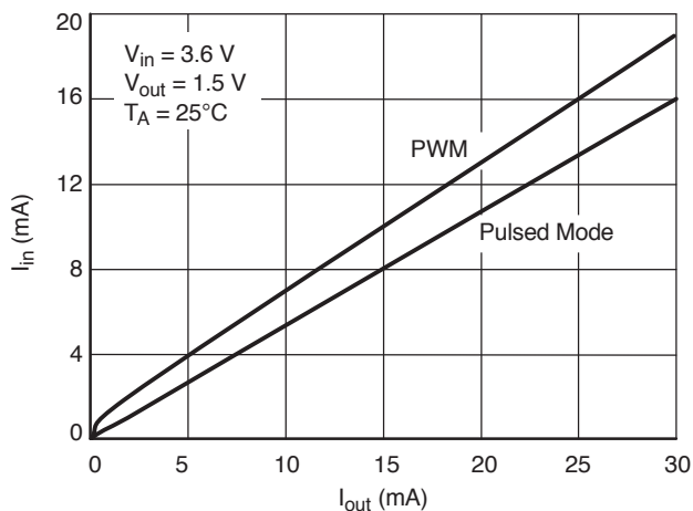
Figure 10. Input Current Comparison
