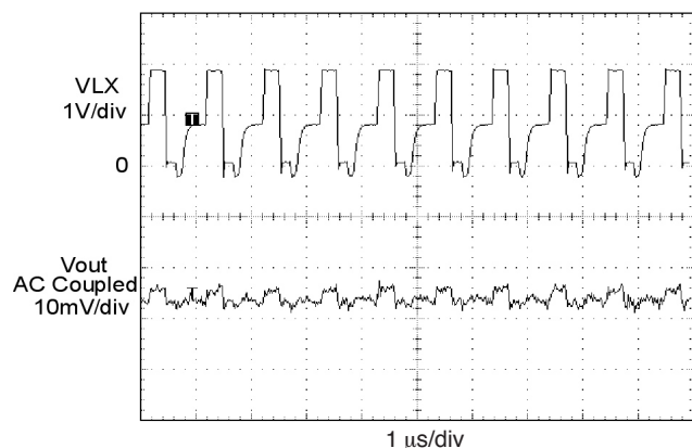
Figure 18. Light-Load PWM Switching Waveform ( V_{in} = 3.6\text{ V} , V_{out} = 1.8\text{ V} , I_{out} = 30\text{ mA} )
