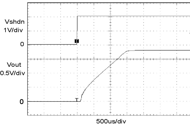
Figure 21. Soft-Start ( V_{in} = 3.6\text{ V} , V_{out} = 1.8\text{ V} , I_{out} = 150\text{ mA} )
