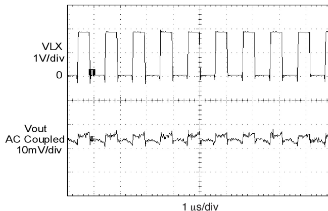
Figure 19. Heavy-Load PWM Switching Waveform ( V_{in} = 3.6\text{ V} , V_{out} = 1.8\text{ V} , I_{out} = 300\text{ mA} )
