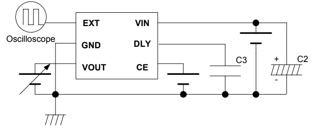
H) Output Delay Time for Protection Circuit
