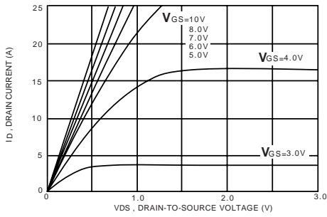
Figure 1. Output Characteristics
