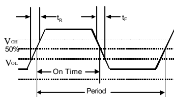
Figure 7. Output Waveform
