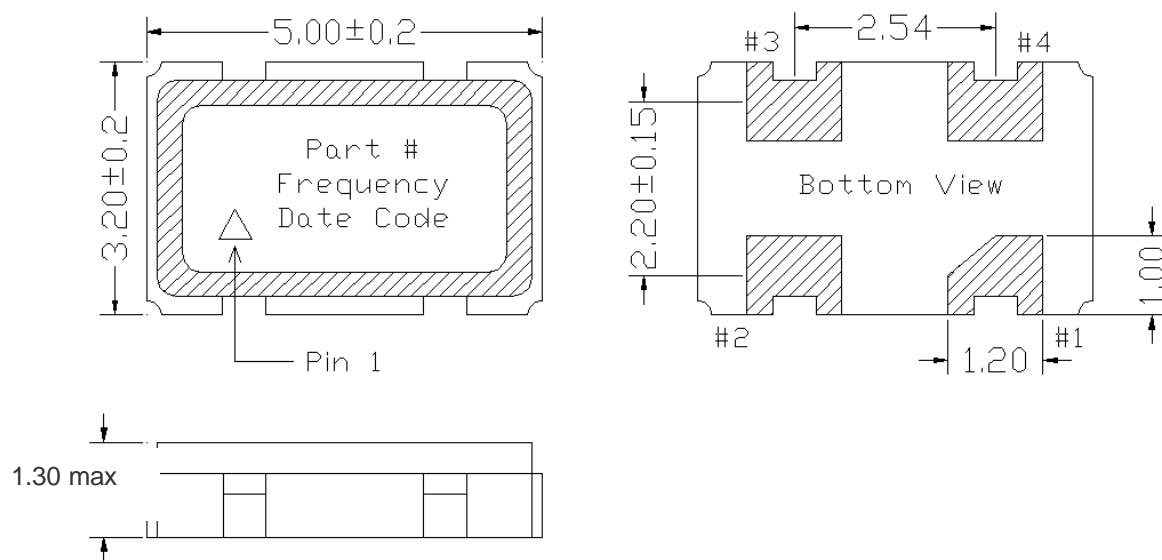
Figure 9, Package drawing
