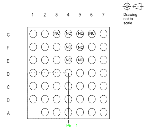
Figure 11.1 : 48BGA pinout (viewed from die side)
