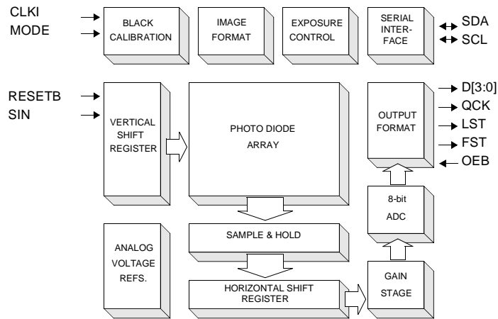
Figure 1.2 : Block Diagram of VV5409 Image Sensor
