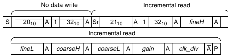
Figure 6.10 : Multiple location read
