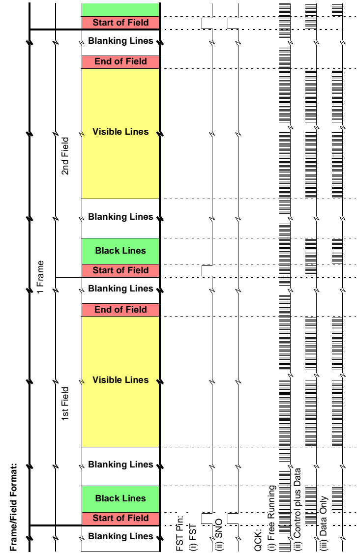
Figure 5.20 : Frame/Field Level Timings for FST and QCK
