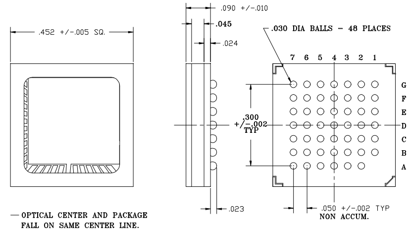
Figure 12.1 : BGA Package dimensions
