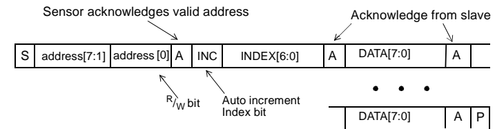
Figure 6.3 : Serial-Interface Data Format
