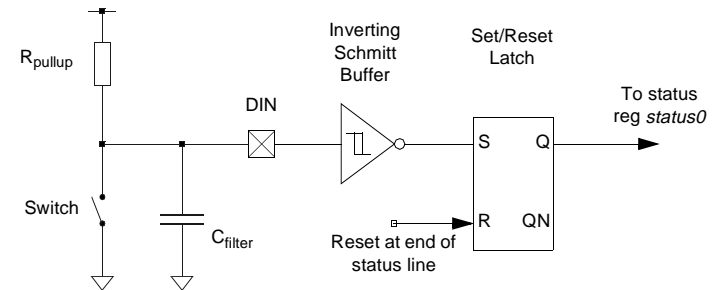
Figure 9.1 : Debounced Switch Input
