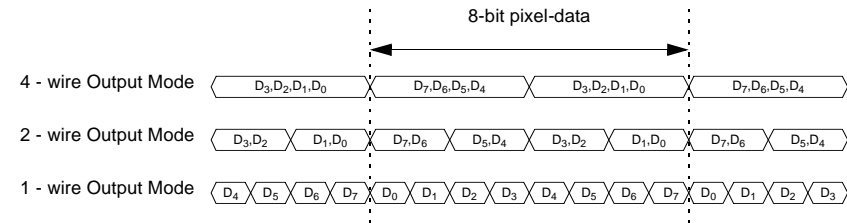
Figure 5.1 : 4-wire, 2-wire and 1-wire Output Modes
