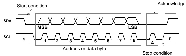
Figure 6.1 : Serial-Interface Data Transfer Protocol
