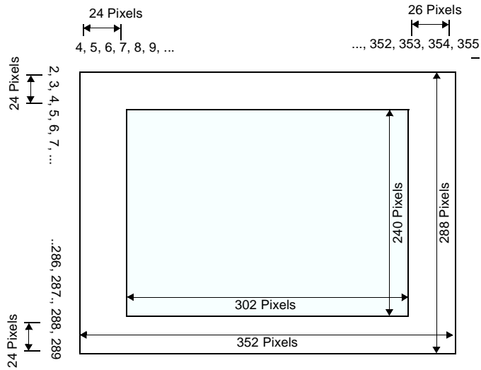
Figure 2.1 : VV5409 Image format with border rows/columns disabled
