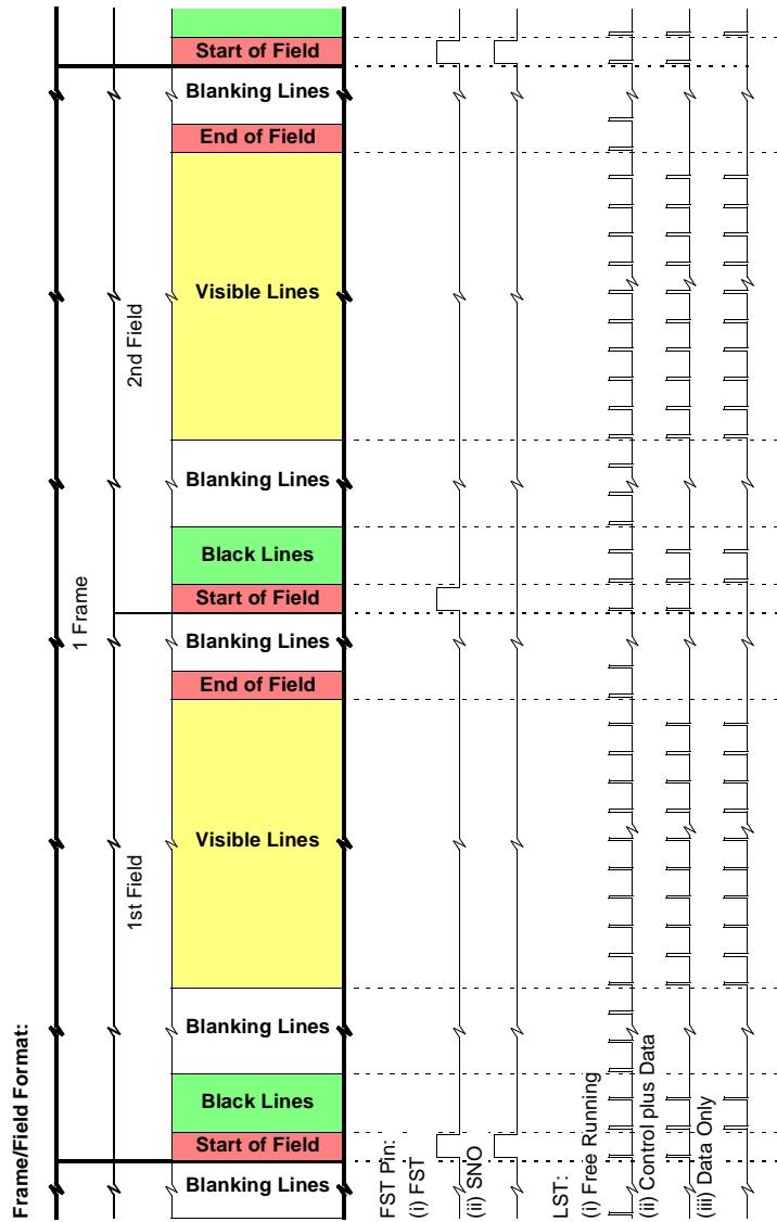
Figure 5.21 : Frame/Field Level Timings for FST and LST
