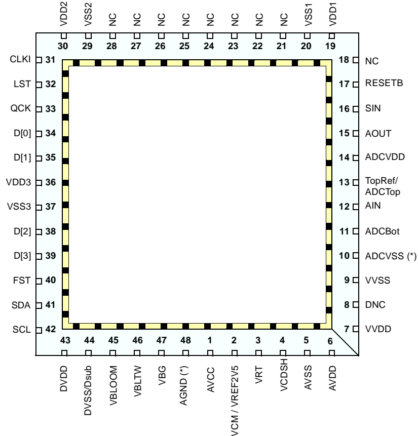
Figure 11.2 : VV5409 Pinout in 48 LCC Package
