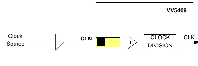
Figure 7.1 : External Clock Source
