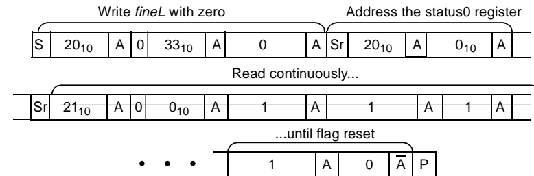
Figure 6.8 : Same location, multiple data read
