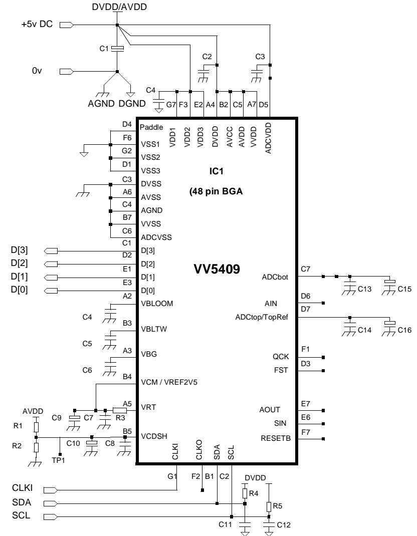
Figure 13.1 : Suggested schematic for VV5409
