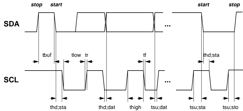
Figure 6.11 : Serial Interface Timing Characteristics
