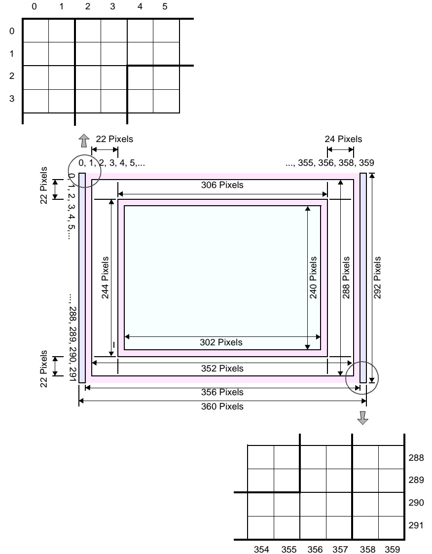
Figure 2.3 : VV5409 Image format with border rows/columns enabled
