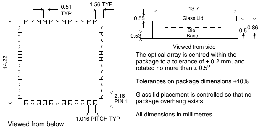
Figure 12.2 : 48LCC package dimensions and optical centering
