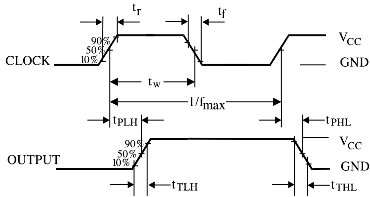
Figure 1. Switching Waveforms
