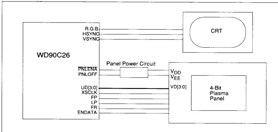
FIGURE 6-22 4-BIT MONOCHROME PLASMA PANEL INTERFACE
