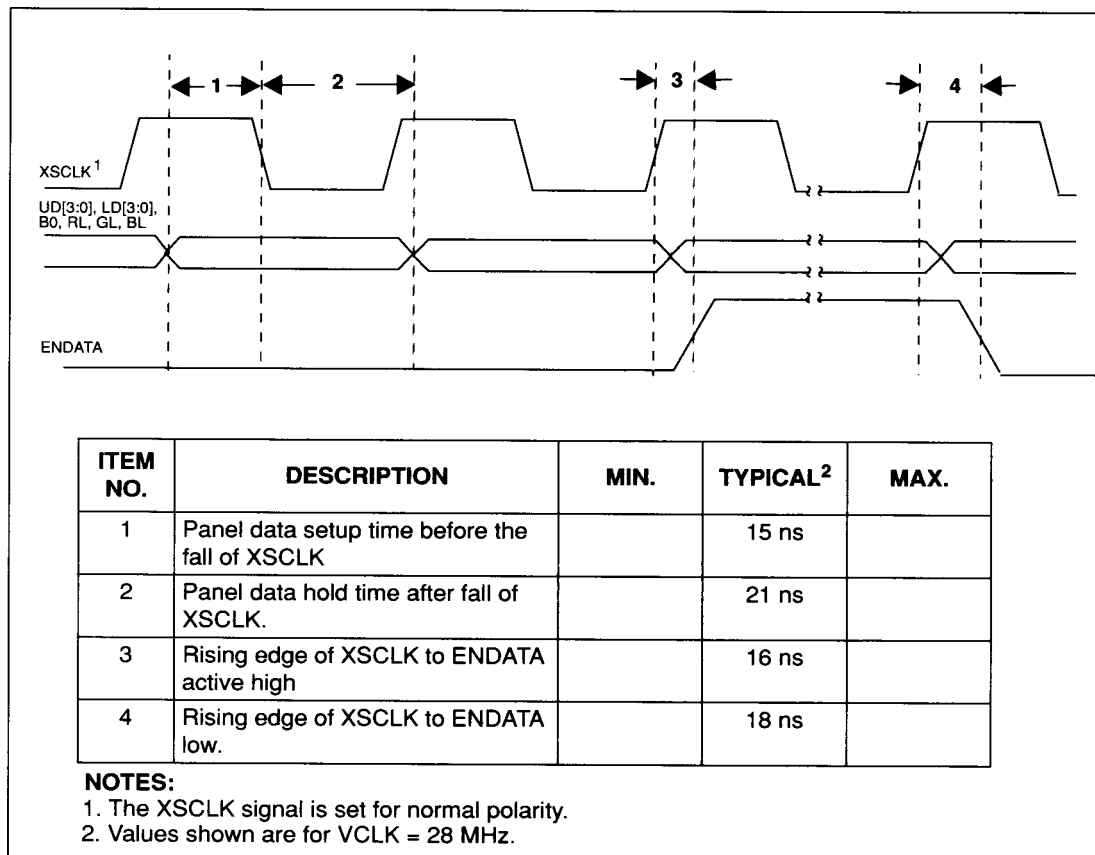
FIGURE 11-8 TFT PANEL AC TIMING
