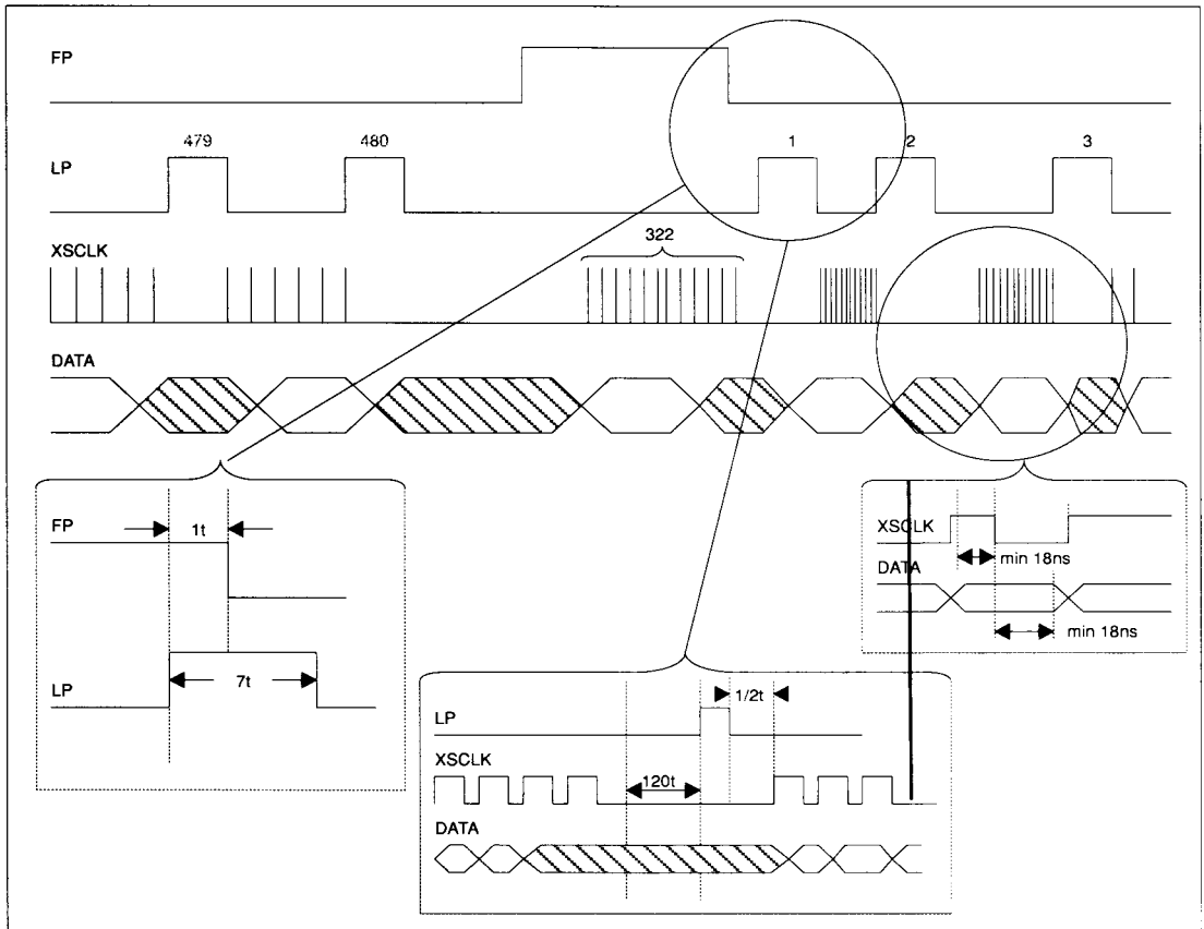
FIGURE 11-7 STN COLOR LCD INTERFACE FUNCTIONAL TIMING
