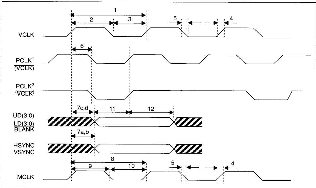
FIGURE 11-1 CLOCK AND EXTERNAL RAMDAC TIMING
