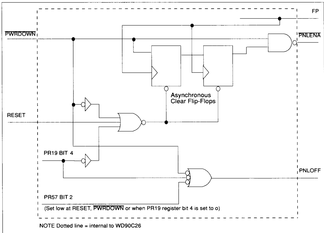
FIGURE 6-12 \overline{\text{P}}\text{NLENA} AND \text{PNLOFF} PANEL PROTECTION SIGNALS
