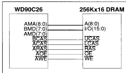
FIGURE 6-8 TYPICAL 256Kx16 DRAM INTERFACE
