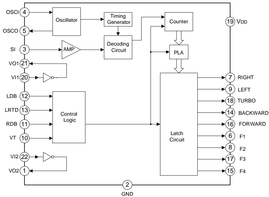
RX-5B Block Diagram
