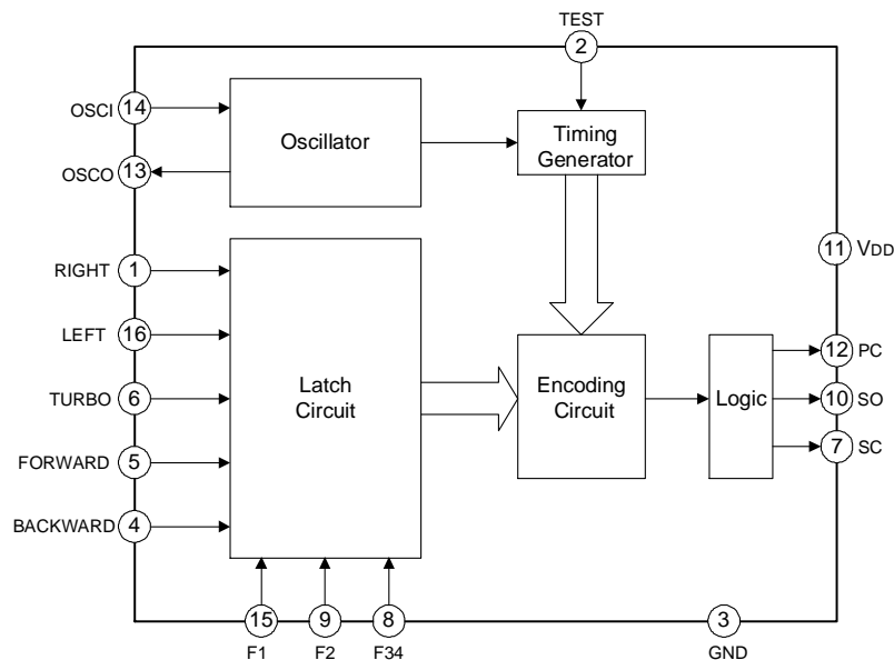
TX-5B Block Diagram
