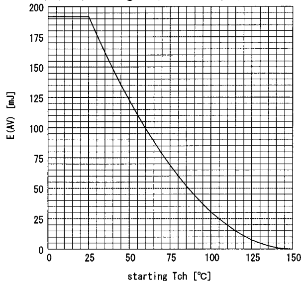
Maximum Avalanche Energy vs. starting Tch E_{(AV)} = f(\text{starting } T_{ch}) : V_{cc} = -12V, I_{(AV)} \ge -5A
