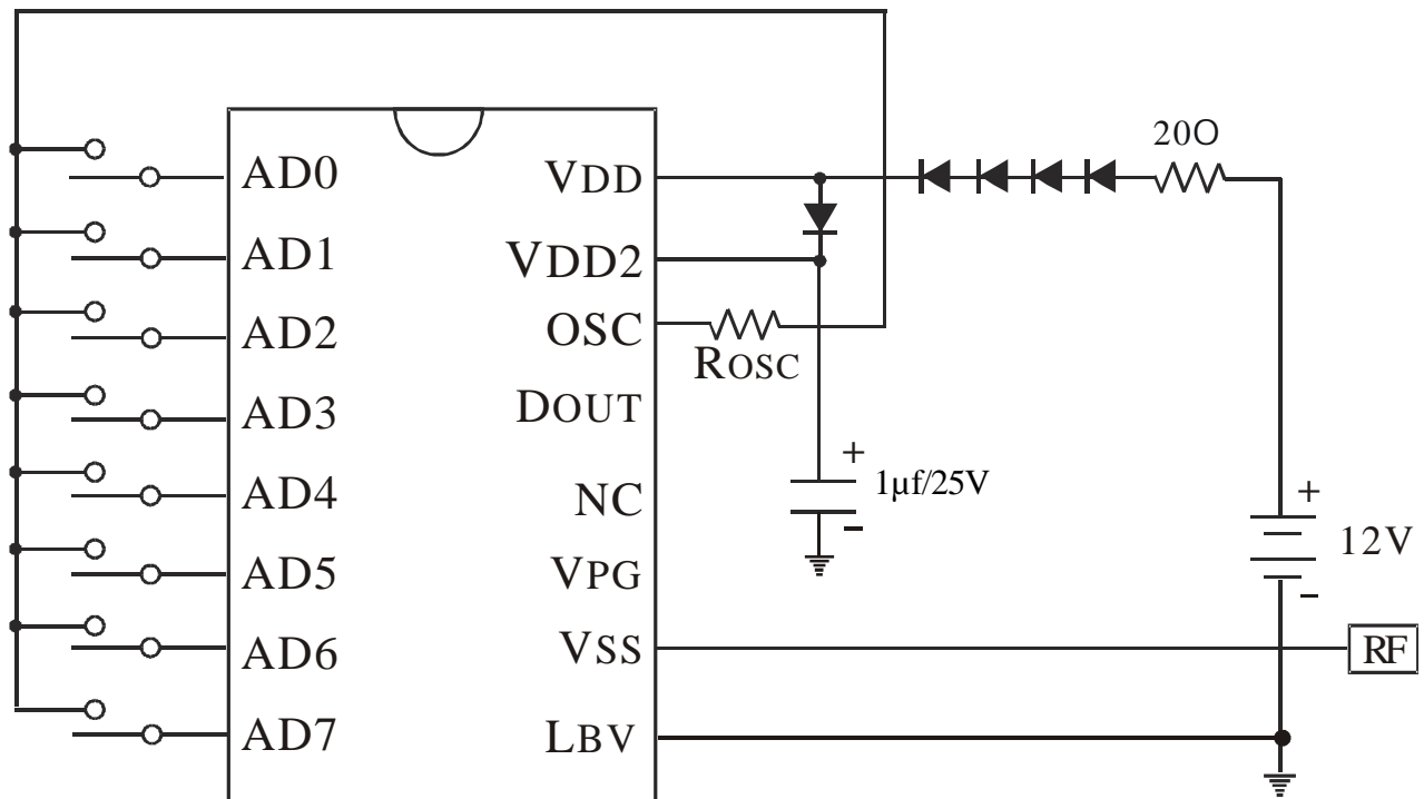
PT2283 (16 Pin)
