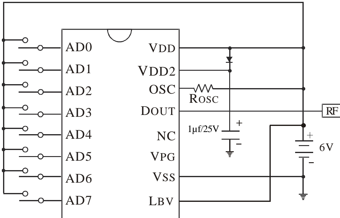
PT2283 (16 Pin)
