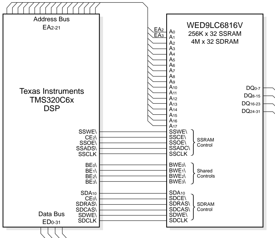
FIG. 17 INTERFACING THE TEXAS INSTRUMENTS TMS320C6x WITH THE WED9LC6816V (256Kx32 SSRAM/4Mx32 SDRAM)
