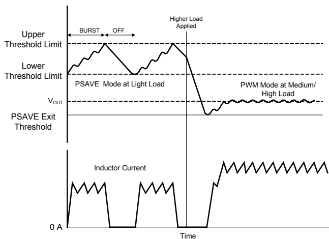
PSAVE Operation
