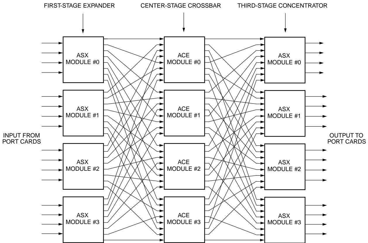
Figure 3. Example 16 x 16 @ 622 Mb/s Switch Fabric (10 Gb/s throughput)
