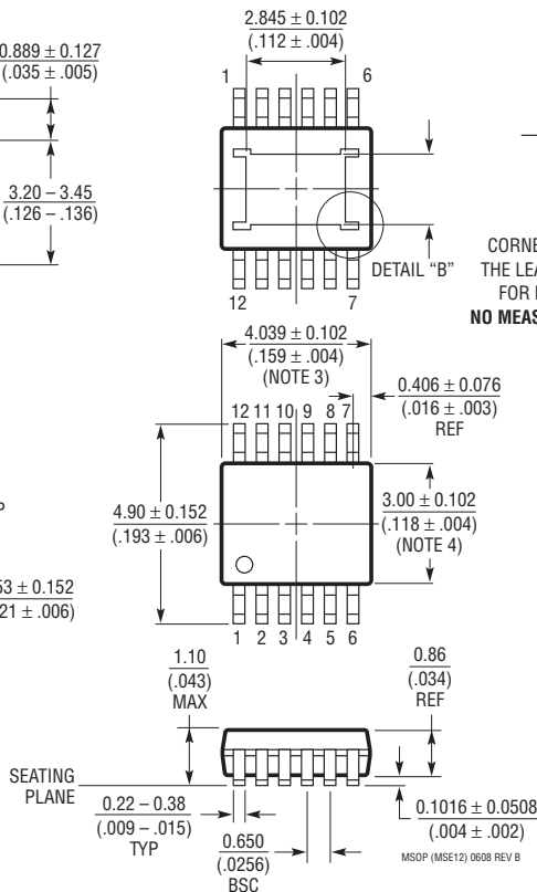
BOTTOM VIEW OF EXPOSED PAD OPTION
