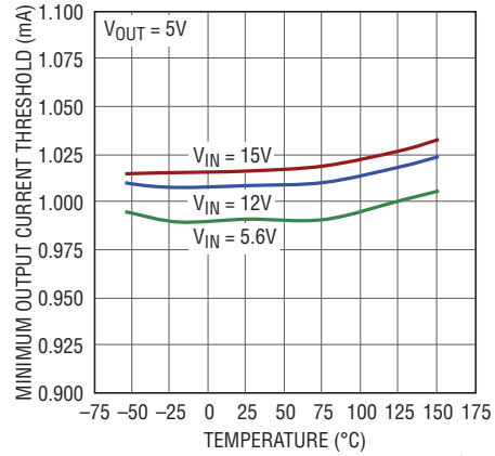
Minimum Output Current Threshold R_{IMIN} = 110k
