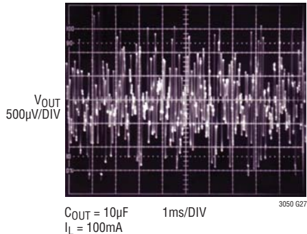
5V 10Hz to 100kHz Output Noise C_{REF/BYP} = 0
