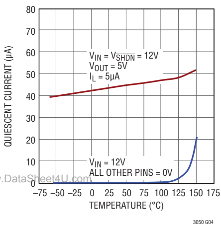
Quiescent Current
