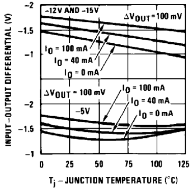
Dropout Voltage
