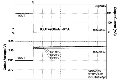
Fig.200. Load Response
