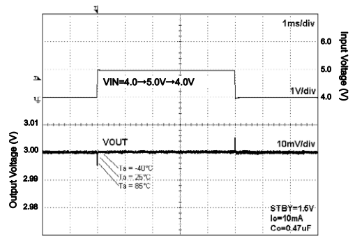
Fig.234. VIN Response
