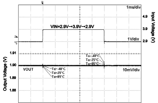
Fig.104. VIN Response
