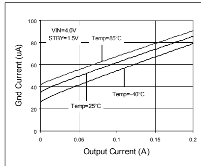
Fig.213. IOUT - IGND
