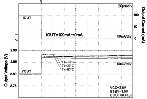
Fig.198. Load Response
