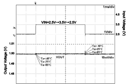
Fig.54. VIN Response
