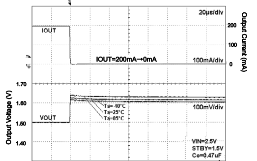
Fig.46. Load Response
