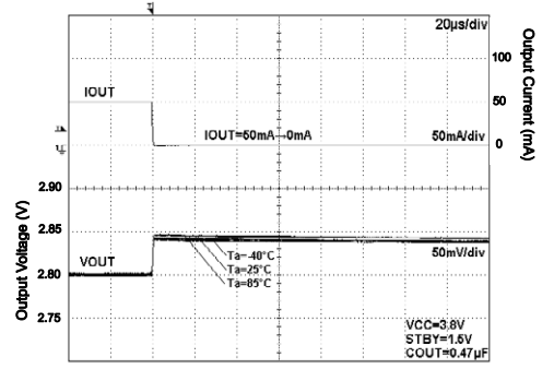
Fig.196. Load Response
