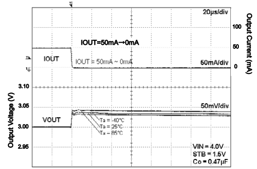
Fig.222. Load Response
