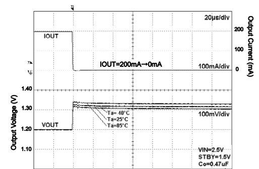
Fig.21. Load Response
