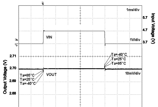
Fig.182. VIN Response
