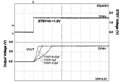
Fig.282. Start Up Time Iout=200mA
