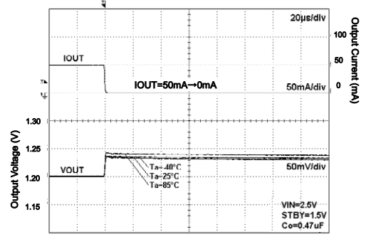
Fig.17. Load Response
