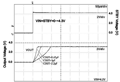
Fig.284. Start Up Time (VIN=STBY) Iout=200mA
