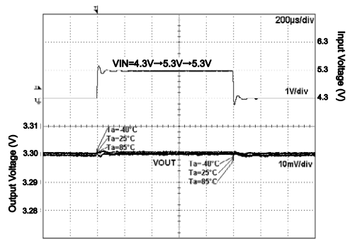
Fig.286. VIN Response
