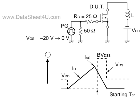
TEST CIRCUIT 1 AVALANCHE CAPABILITY
