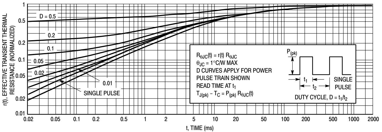
Figure 16. Thermal Response
