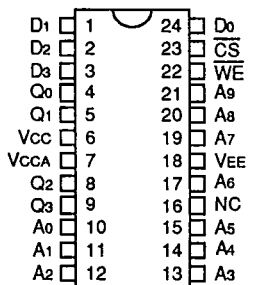
TOP VIEW 2760 drw 02
