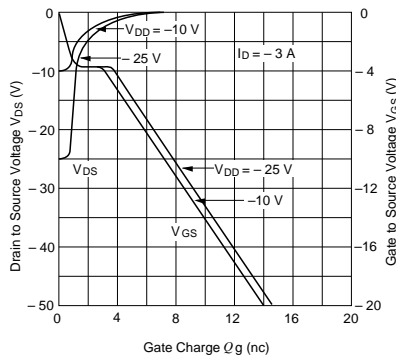
Switching Characteristics
