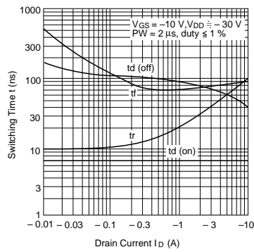
Switching Characteristics
