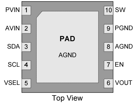
Figure 3. MLP10, 3x3mm
