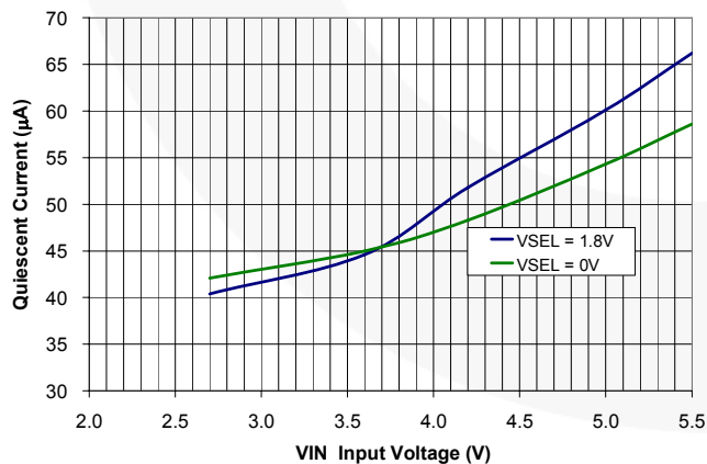
Figure 15. Quiescent Current, I_{LOAD} = 0 , EN = 1.8V
