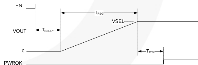
Figure 37. Soft-Start Timing
