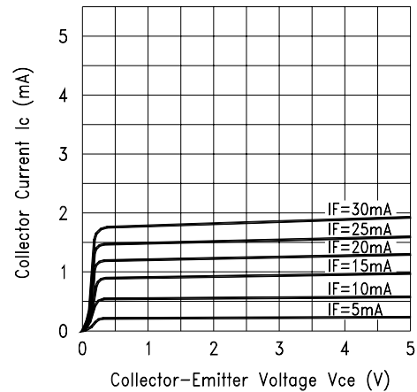
Fig.2 COLLECTOR CURRENT VS. COLLECTOR VOLTAGE
