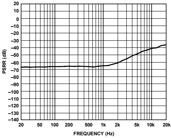
Figure 16. Power Supply Rejection Ratio (PSRR) vs. Frequency
