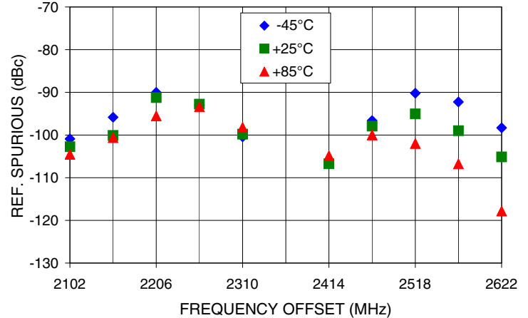
REFERENCE SPURIOUS Vs FREQ. OFFSET @ Fcar = 2362MHz
