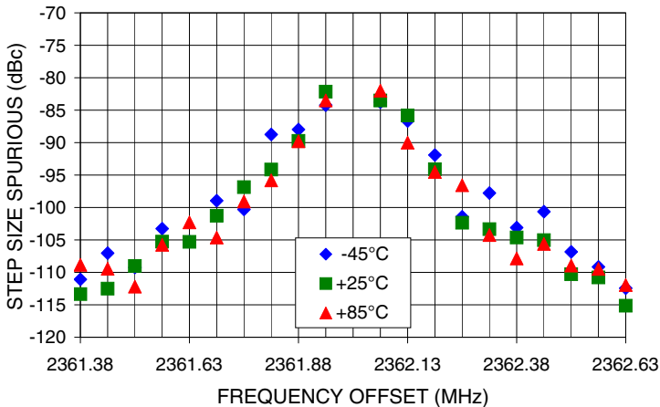
0.5 STEP SIZE & STEP SIZE SPURIOUS Vs FREQ. OFFSET @ F car = 2362MHz
