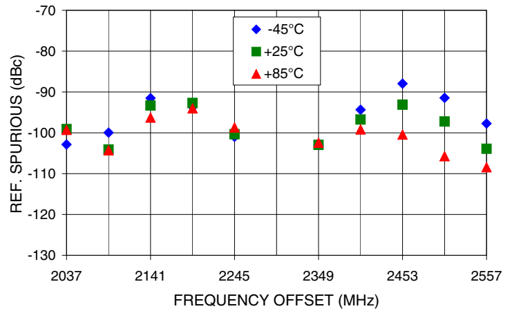
REFERENCE SPURIOUS Vs FREQ. OFFSET @ Fcar = 2297MHz
