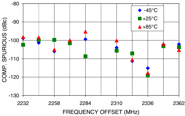
COMPARISON SPURIOUS Vs FREQ. OFFSET @ Fcar = 2297MHz
