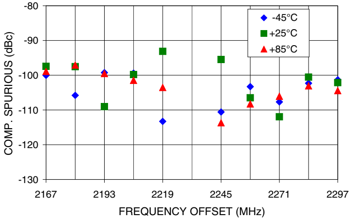
COMPARISON SPURIOUS Vs FREQ. OFFSET @ Fcar = 2232MHz
