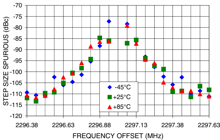
0.5 STEP SIZE & STEP SIZE SPURIOUS Vs FREQ. OFFSET @ F car = 2297MHz
