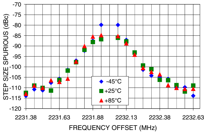
0.5 STEP SIZE & STEP SIZE SPURIOUS Vs FREQ. OFFSET @ F car = 2232MHz
