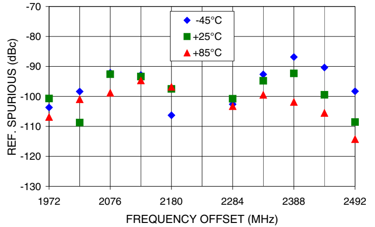
REFERENCE SPURIOUS Vs FREQ. OFFSET @ Fcar = 2232MHz
