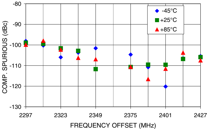
COMPARISON SPURIOUS Vs FREQ. OFFSET @ Fcar = 2362MHz
