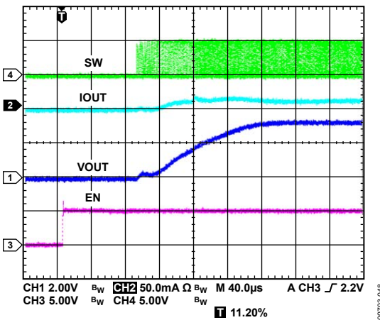
Figure 5. BUCK2 Startup, V_{OUT2} = 3.3\text{ V} , I_{OUT2} = 10\text{ mA}
