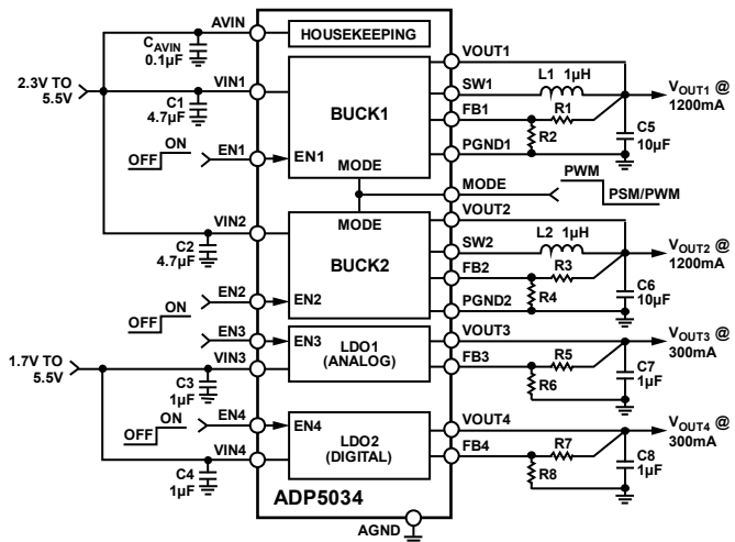
Figure 53. ADP5034 Adjustable Output Voltages with Enable Pins
