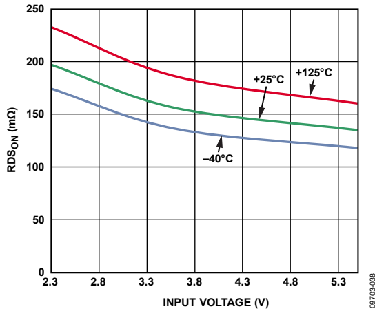
Figure 33. PMOS RDS ON vs. Input Voltage Across Temperature
