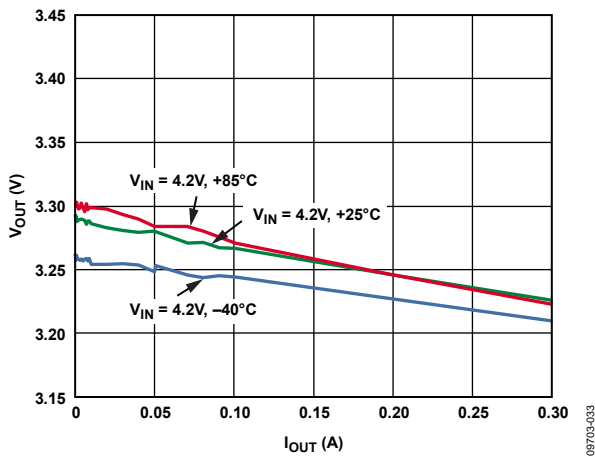
Figure 34. LDO Load Regulation Across Temperature, V_{IN3} = 3.3\text{ V} , V_{OUT3} = 2.8\text{ V}
