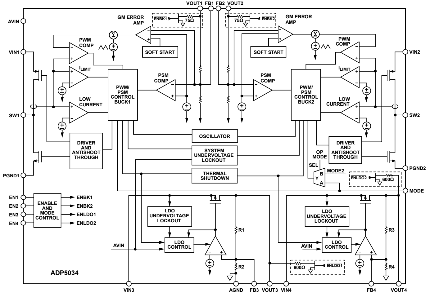
Figure 45. Functional Block Diagram
