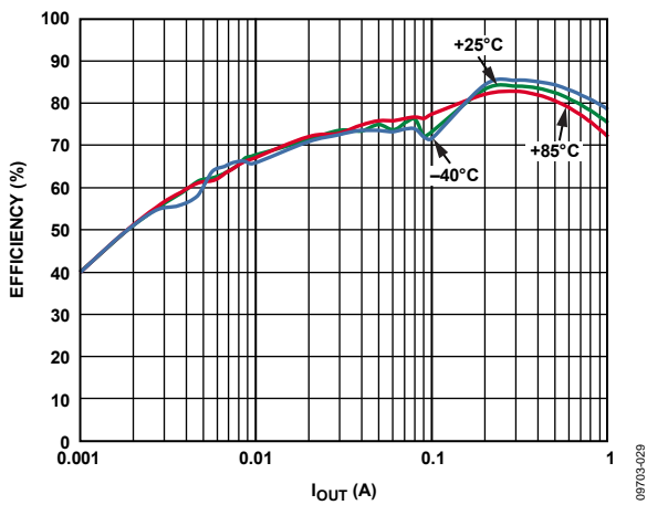
Figure 17. BUCK2 Efficiency vs. Load Current, Across Temperature, V_{OUT1} = 0.8\text{ V} , Auto Mode
