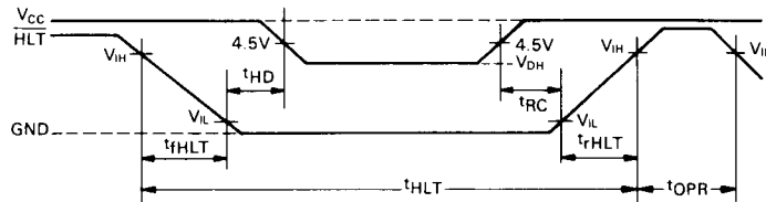
Figure 19 Halt Timing
