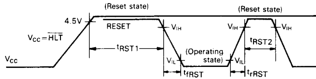
Figure 17 RESET Timing
