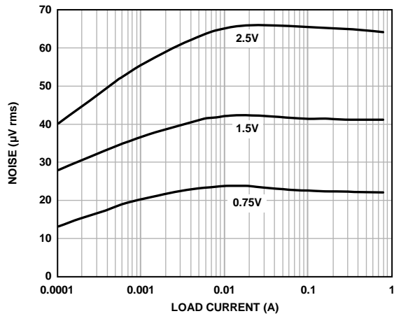
Figure 18. Noise vs. Load Current and Output Voltage
