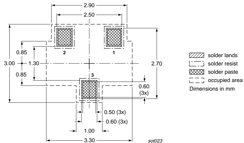
Fig 13. Reflow soldering footprint SOT23 (TO-236AB)
