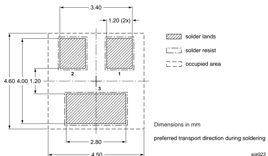
Fig 14. Wave soldering footprint SOT23 (TO-236AB)
