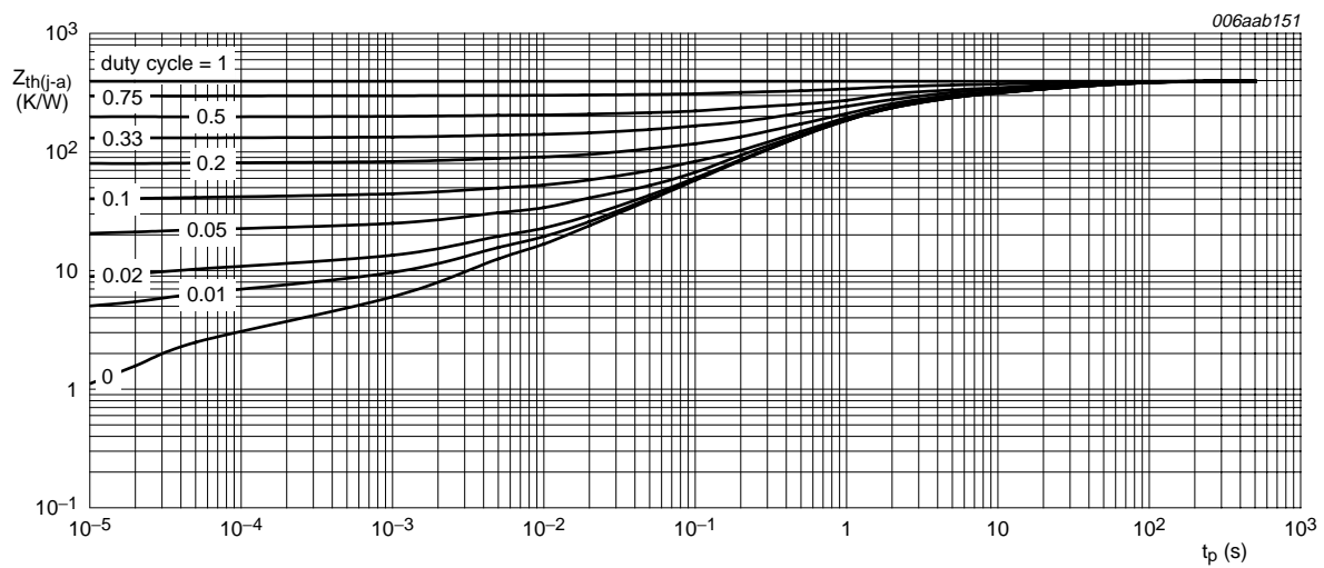
Fig 2. Transient thermal impedance from junction to ambient as a function of pulse duration for SOT23 (TO-236AB)
