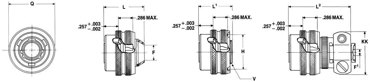
*JT06P-XX-XXX (MS27336P) *JTN06P-XX-XXX
