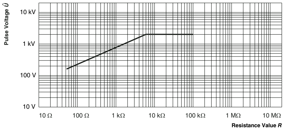
1.2/50 Pulse Pulse load rating in accordance with IEC 60115-1, 4.27; 1.2 \mu s/50 \mu s; 5 pulses at 12 s intervals; for permissible resistance change 0.5 %
