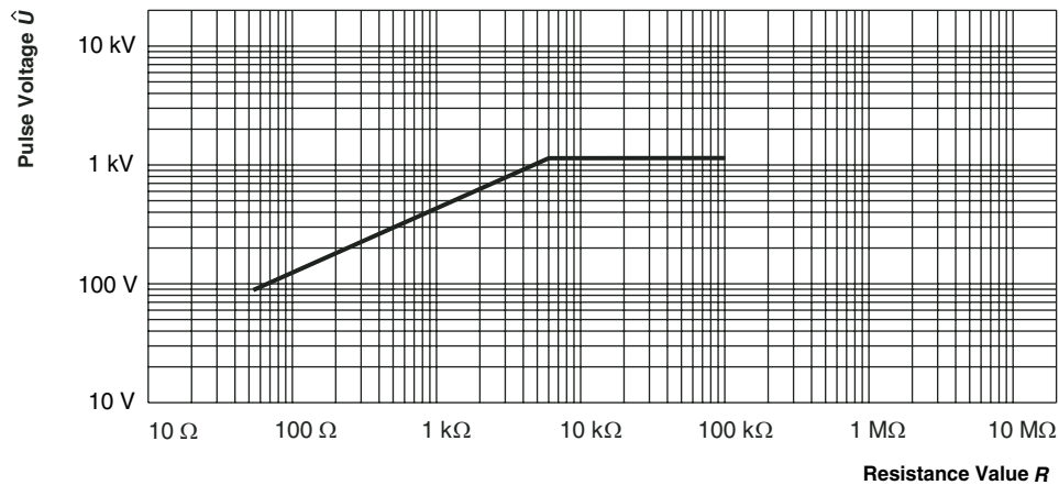
10/700 Pulse Pulse load rating in accordance with IEC 60115-1, 4.27; 10 \mu s/700 \mu s; 10 pulses at 1 min intervals; for permissible resistance change 0.5 %
