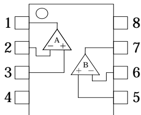
NJM14558/14558M/14558E NJM14558V/14558R
