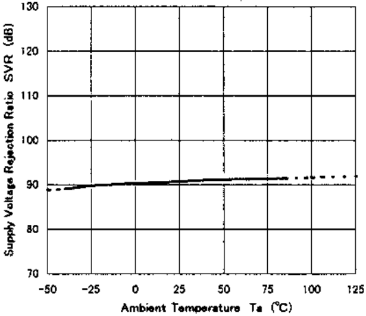
NJM14558 Supply Voltage Rejection Ratio vs. Temperature
