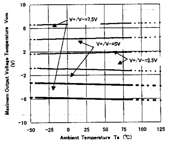
NJM14558 Maximum Output Voltage Swing vs. Temperature
