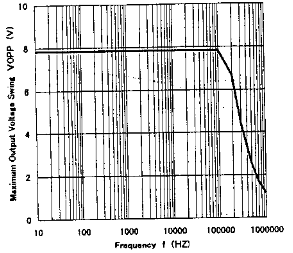
NJM14558 Maximum Output Voltage Swing vs. Frequency
