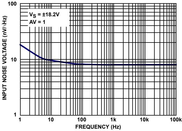
FIGURE 57. CHARACTERIZED INPUT NOISE VOLTAGE
