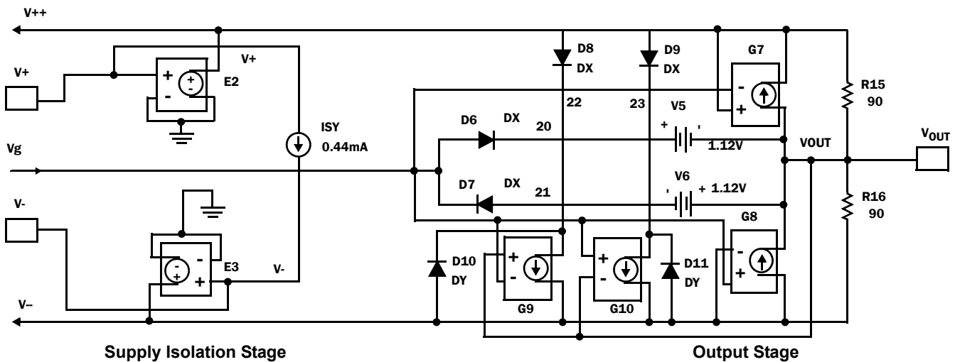
FIGURE 55. SPICE SCHEMATIC
