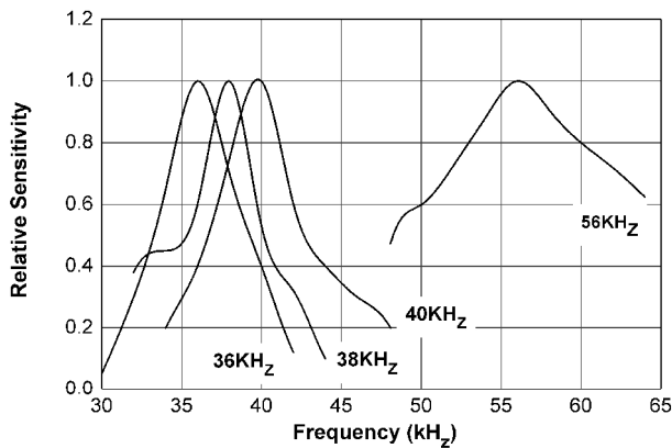
Fig.8 Relative Sensitivity vs. Frequency
