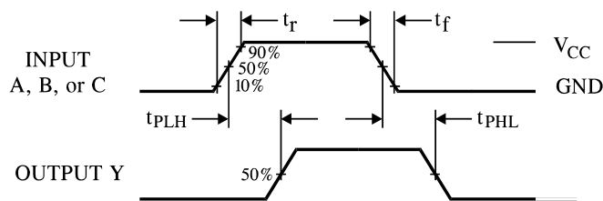
Figure 1. Switching Waveforms
